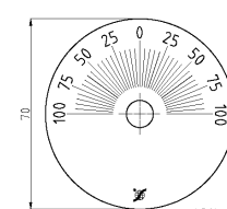
Scale 2x90° 100-0-100 Ø70 Base silver, text black
