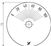
Scale 120° 0-100 Ø70 Base silver, text black
