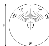
Scale 2x60° 100-0-100 Ø70 Base silver, text black
