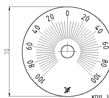
Scale 2x90° 100-0-100 Ø70 Base silver, text black
